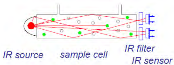
fig. 1 example set-up with dual channel sensor
