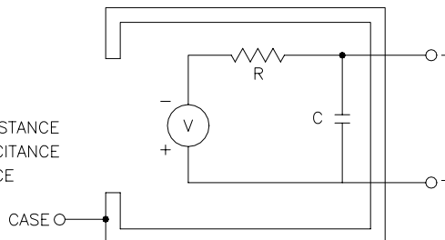
Equivalent Circuit Single Element Thermopile Detector
